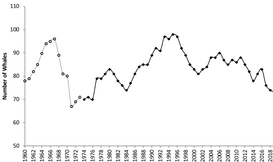
Figure 2.1.a. Population size and trend of Southern Resident killer whales, 1960-2019. Data from 1960-1973 (open circles, gray line) are number projections from the matrix model of Olesiuk et al. (1990). Data from 1974-2019 (diamonds, black line) were obtained through photo-identification surveys of the three pods (J, K, and L) in this community and were provided by the Center for Whale Research (unpublished data) and NMFS (2008). Data for these years represent the number of whales present at the end of each calendar year.
