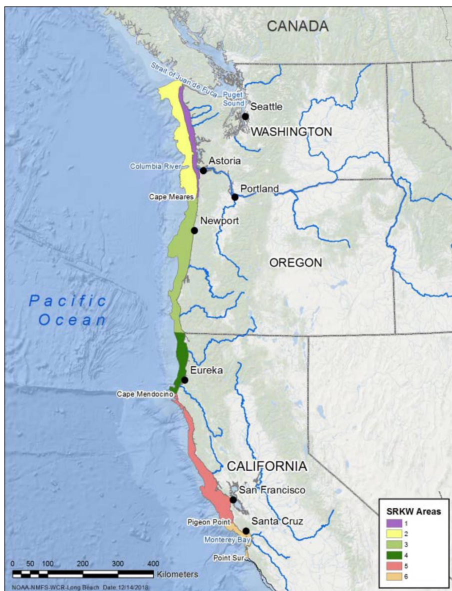
Figure 2.2.b. Specific areas containing essential habitat features (Figure 9 reproduced from NMFS 2019b).
