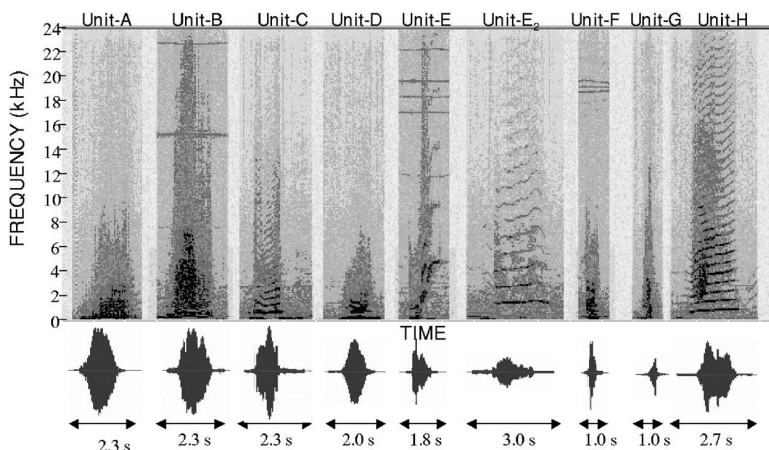
FIG. 2. Spectrogram and waveform representation of the nine units contained in the humpback whale songs during the winter season in Hawaiian waters in 2002. The units were from the recordings of several whales and were chosen because they showed the characteristics of the unit most clearly.
