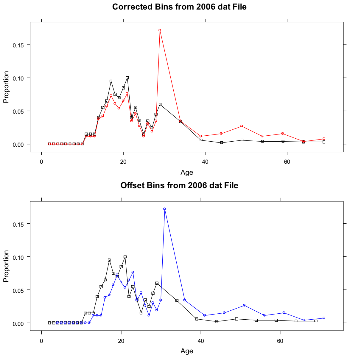
Figure 5. 2001 Washington hook-and-line age compositions used in the 2006 coast-wide base model (circles) and the 2007 base model (squares).
