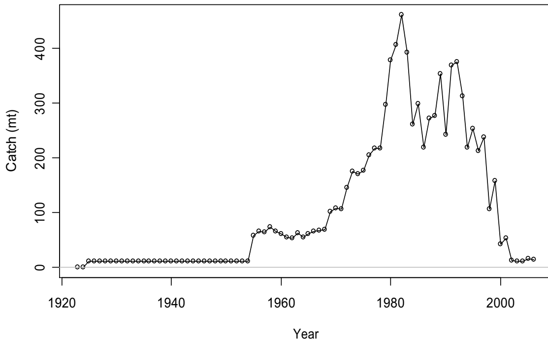
Figure 1. Reconstructed historical catch (mt) by year and fleet, 1925-2006.
