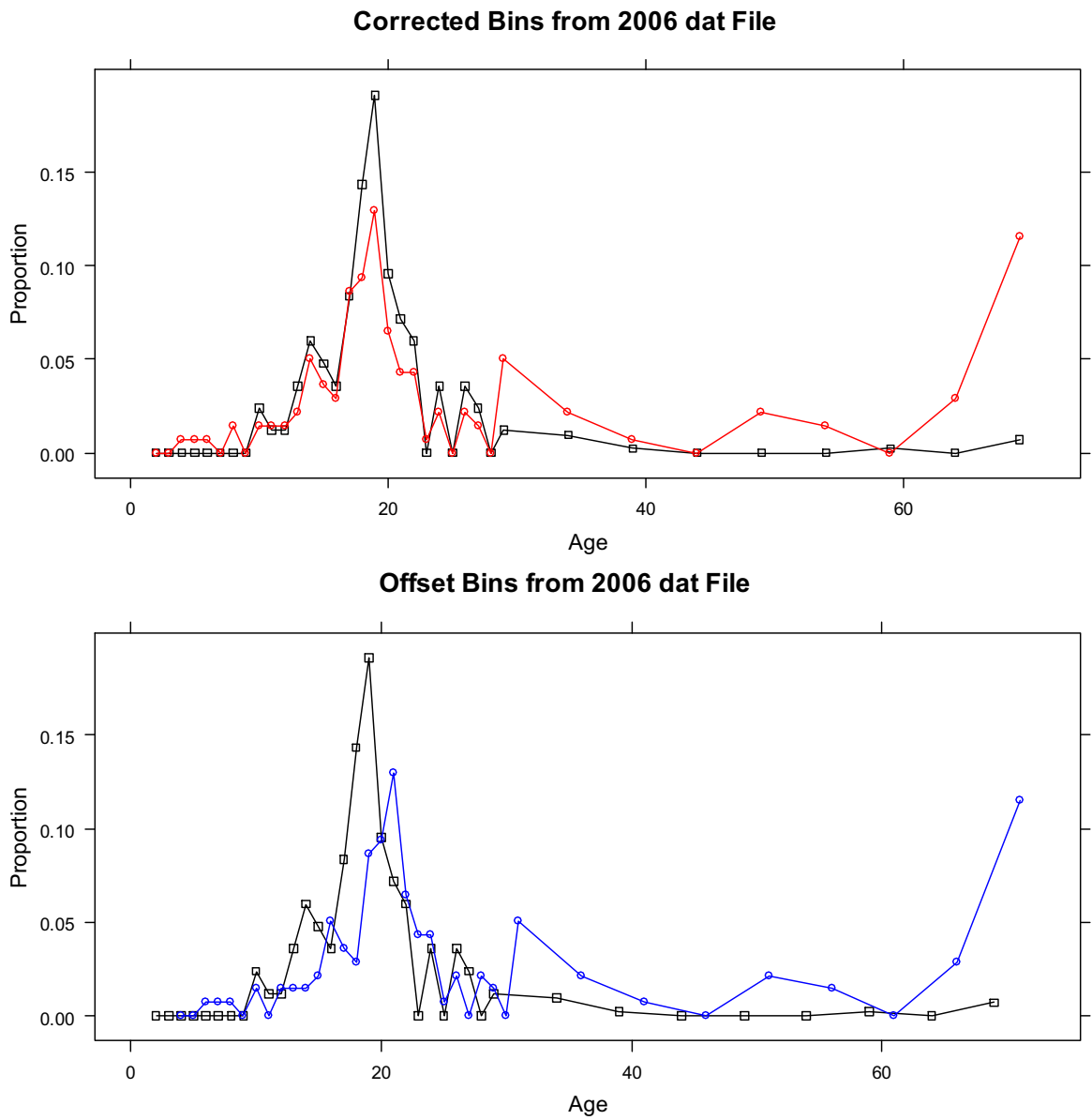
Figure 3. 2002 Washington hook-and-line age compositions for the 2006 coast-wide base model (circles) and the 2007 base model (squares).
