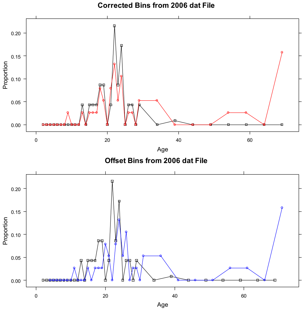
Figure 4. 2004 Washington hook-and-line age compositions for the 2006 coast-wide base model (circles) and the 2007 base model (squares).
