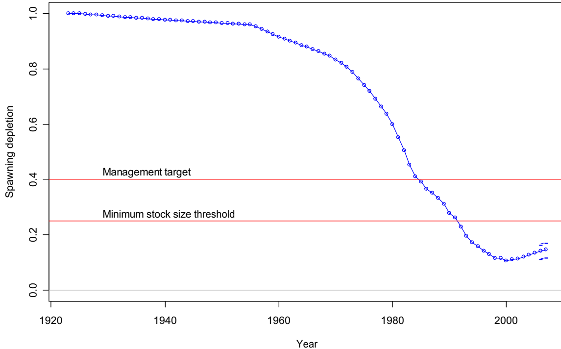
Figure ES4. Time-series of estimated depletion level, 1925-2007 with approximate asymptotic 95% confidence interval for 2006 and 2007, using the 2007 base model.
