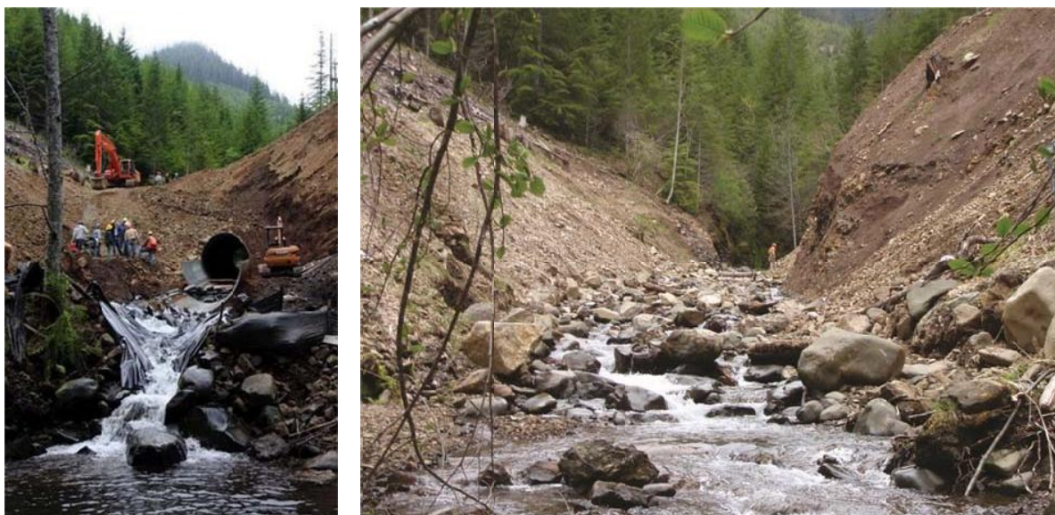
Figure 4-1. An example of culvert and road fill removal on a tributary drainage to the upper South Fork (USFS 2017).
