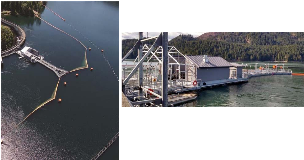
Figure 4-10. Left – Aerial photo showing the Floating Surface Collector (FSC) in place at the lower end of the upper reservoir and attached to the upstream face of the dam. The guide nets, arranged roughly in a “W” shape to help guide downstream emigrants to the upstream opening of the FSC, are also seen. Right – The FSC structure as seen from the rim of the dam.
