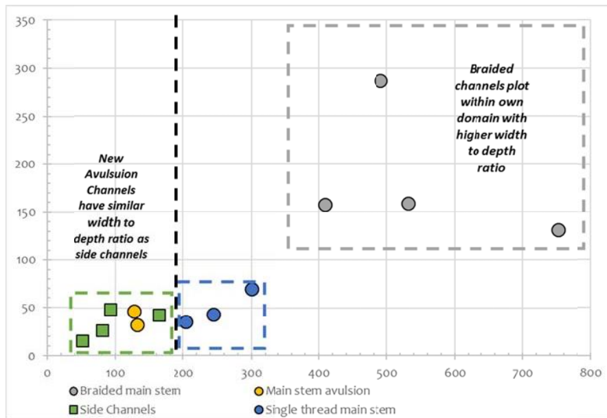
Figure 4-18. Channel width to depth ratio versus unvegetated channel width. Note the two separate domains in which data group, one for side channels and single thread mainstem channels and one for braided channel reaches. From NSD (2017).
