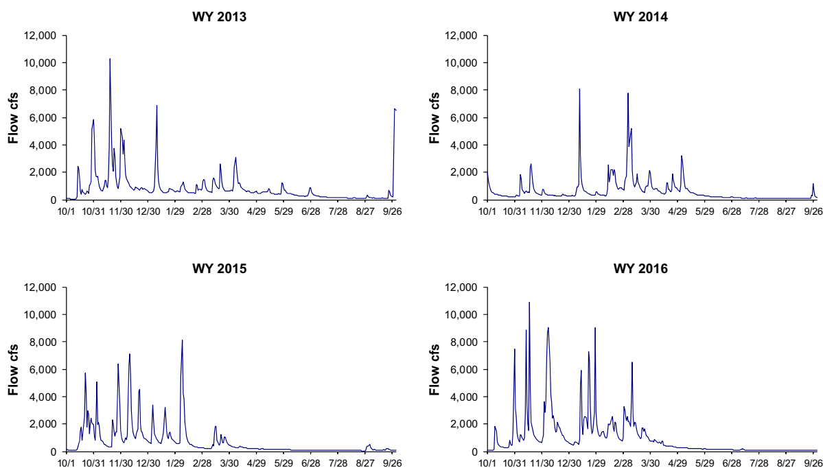
Figure 4-16. Hydrographs for the South Fork below the gorge for water years (WY) 2013-2016 (USGS 12060500). See Figure 4.12 for location.
