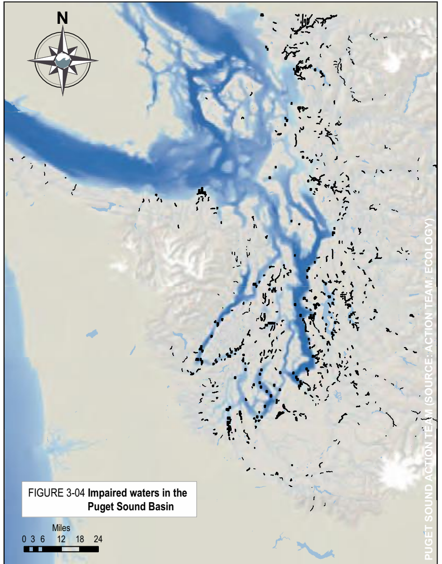
FIGURE 3-04: (right) Every two years, the Department of Ecology assesses the quality of the surface waters of Washington State. Water bodies that do not meet the state's water quality standards because of human-caused problems are identified as impaired and assigned a category for further study and clean up. In 2004, there were approximately 1,474 listings of impaired waters in Puget Sound's fresh and marine waters. Most of the impairments are the result of toxic contamination, pathogens, low dissolved oxygen and high temperatures. Source: Action Team; Ecology.
