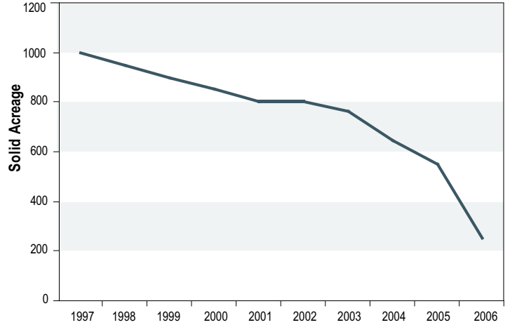
FIGURE 7-19: Since 2004, areas of Puget Sound covered by spartina have dropped from 645 acres to 250 acres. Source: Agriculture.
