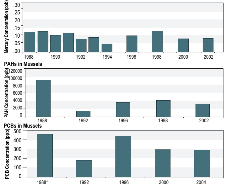
FIGURE 4-08: The National Oceanic and Atmospheric Administration's Mussel Watch program has collected data on contaminants in mussels since 1984. PCB and PAH concentrations have generally declined; mercury levels have stayed fairly stable. Source: NOAA.
