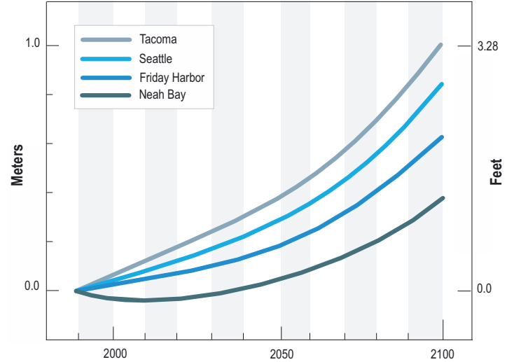
FIGURE 9-27: Future sea level rise scenarios for various locations in Puget Sound are shown. These sea level rise curves take into account projected global sea level rise, the increased rate projected for the NE Pacific and the sinking of local land. The degree of sea level rise projected at Tacoma for 2050 (about 1.2 feet or 0.4 m) would not occur at Seattle until around 2060 and at Friday Harbor until around 2080. Given continued uncertainty, the sea level rise scenarios could be 20 percent to nearly 200 percent of the mid-range scenarios depicted. Source: Uncertain Future: Climate Change and Its Effects on Puget Sound . Action Team, 2005.
