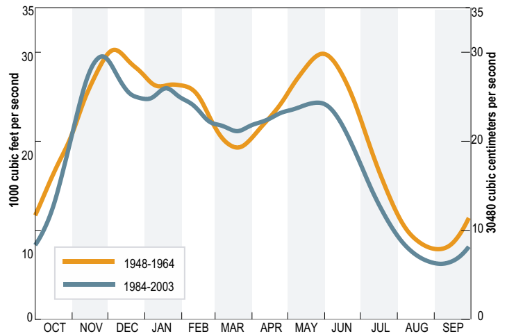
FIGURE 9-28 Average daily freshwater flow into Puget Sound 1948-2003
