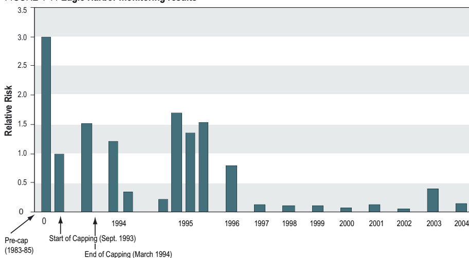
FIGURE 4-11 Eagle Harbor monitoring results
