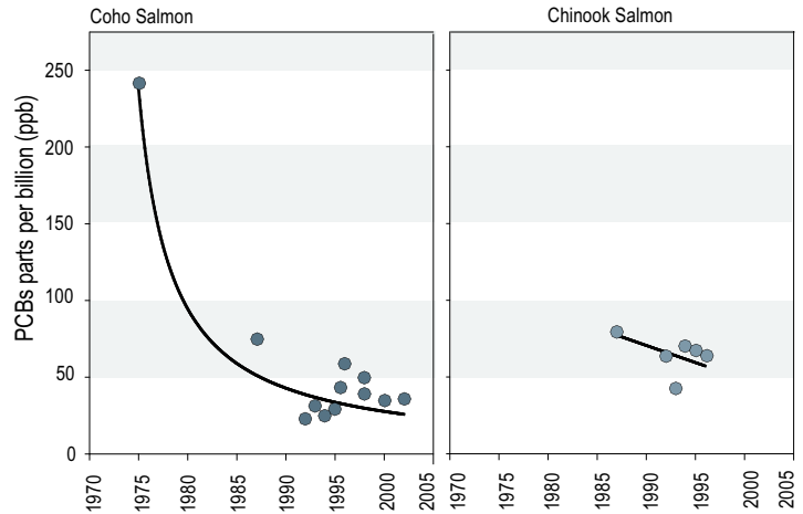
FIGURE 4-07 PCB trends in Puget Sound salmon 1970-2005
