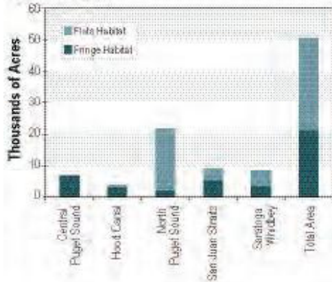
FIGURE 7-18 Estimated native eelgrass by type and region
