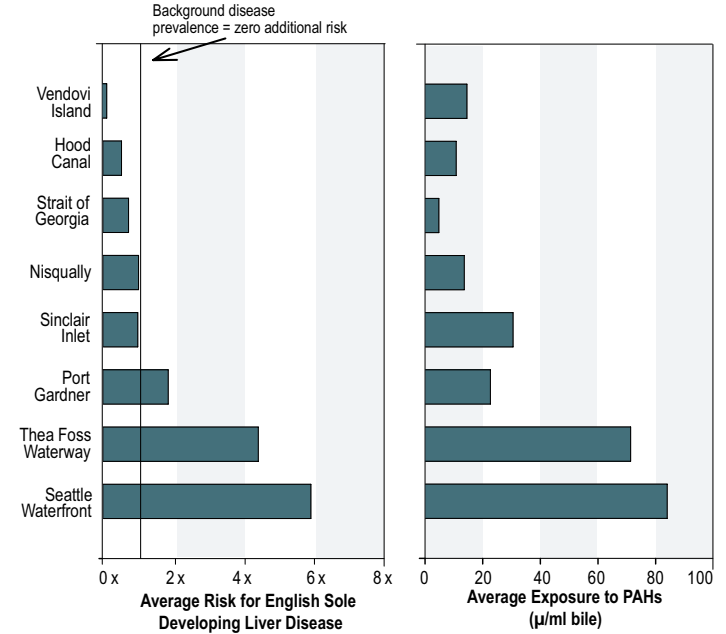
FIGURE 4-10: The risk of English sole developing liver disease was assessed at eight long-term monitoring stations. Their exposure to PAHs was determined by using a biomarker phenanthrene, which is a chemical released by the liver into bile when the fish is exposed to PAHs. This is measured as micrograms per milliliter of phenanthrene in bile (µ/ml bile). Risks were averaged over a 17-year period, and PAH exposure was averaged over an eight-year period. Source: WDFW
