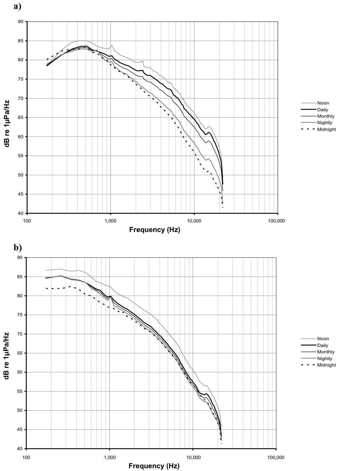
Figure 3. Spectrum levels in Haro Strait in a) July 2005 and b) November 2005 (based on Figure 7 and Figure 8 in Veirs and Veirs 2005).
