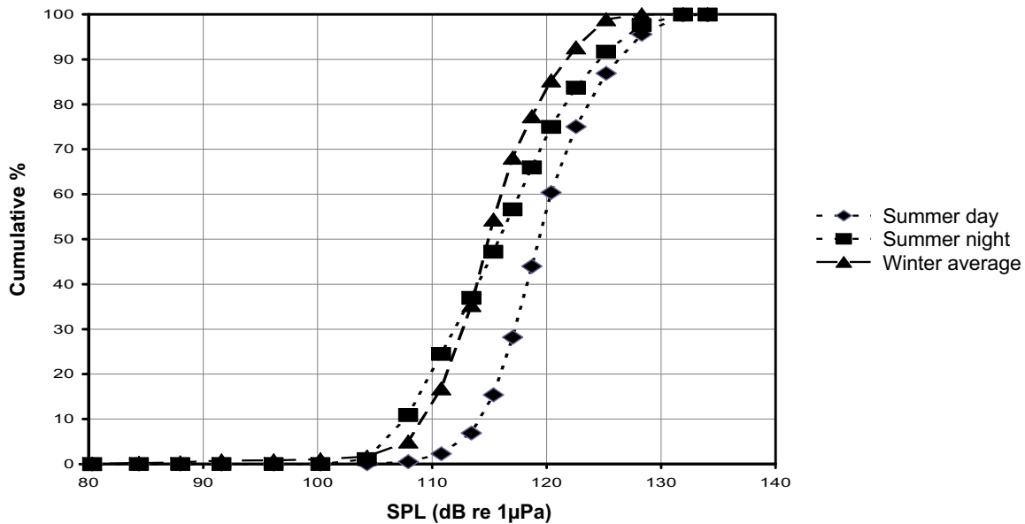
Figure 2. Cumulative distributions of 2-second average SPLs (0.1–15 kHz). Summer day includes SPL measurements during the hours of 0800–2000 and summer night includes SPL measurements from the other 12 of the 24 hour cycle (based on Figure 6 of Veirs and Veirs 2005).
