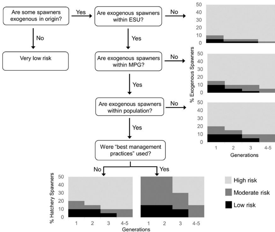
Figure 2. Risk of maintaining natural patterns of gene flow associated with spawner composition and number of generations (modified from ICTRT 2007). Exogenous fish are all hatchery-origin fish, and non-normative strays of natural origin.
