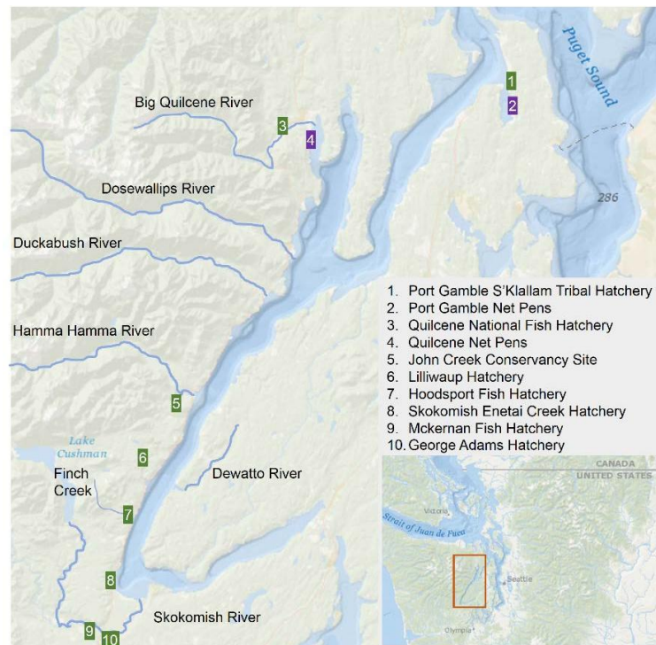
8 9 Figure 1. Location of hatchery programs and major Hood Canal tributaries included in this 10 analysis.
