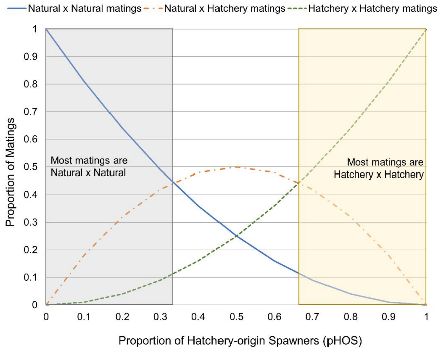
3 Figure 3. Relative proportions of mating types as a function of proportion of hatchery- 4 origin fish on the spawning grounds (pHOS).
