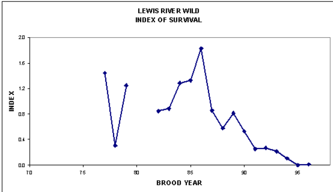
Figure 1. Early ocean survival rate index for Lewis River wild chinook (LCR ESU)
