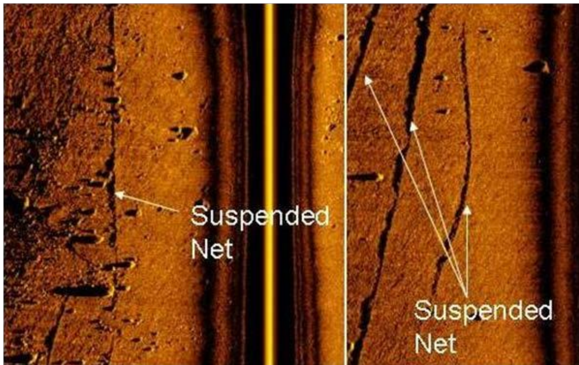
Figure 15. Sidescan sonar images of derelict nets located on Point Roberts Reef of the San Juan basin. Suspended nets have a larger acoustic shadow than nets flush with the bottom. Image used by permission of Natural Resource Consultants (NRC).
