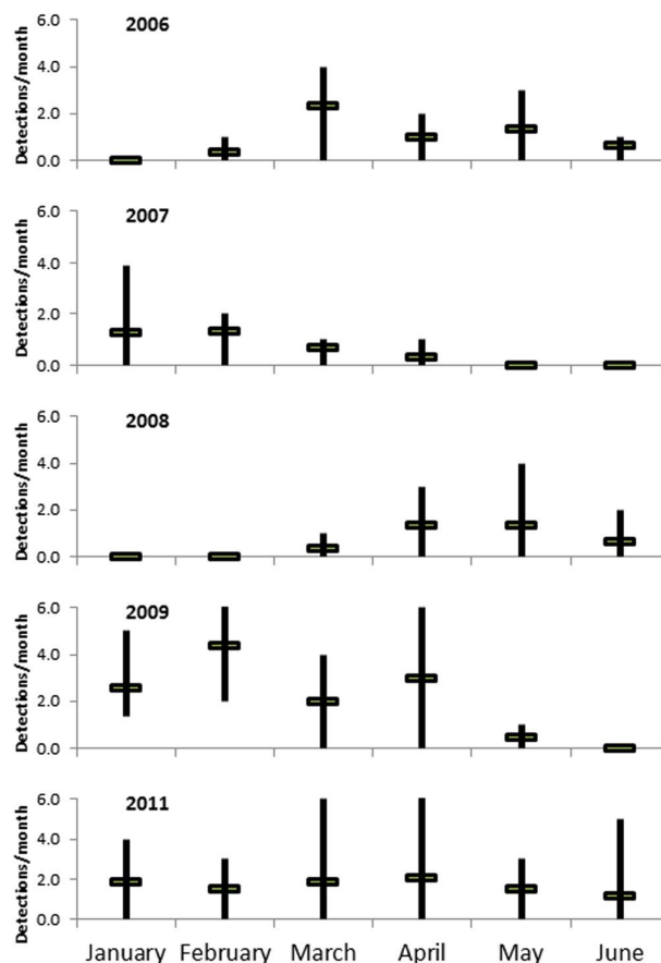
FIG. 4. (Color online) Mean number of SRKW detections/month (horizontal bar) and range in number of detections (vertical bar) by year at all recorder locations.
