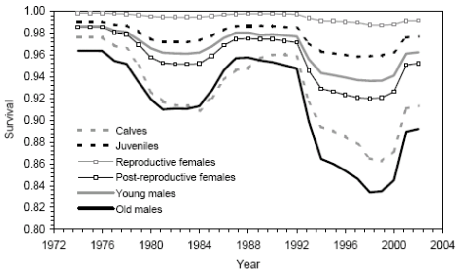
Figure 11. Model-averaged estimates of survival by age and sex category for the entire Southern Resident population, 1974-2002 (Krahn et al. 2004a).
