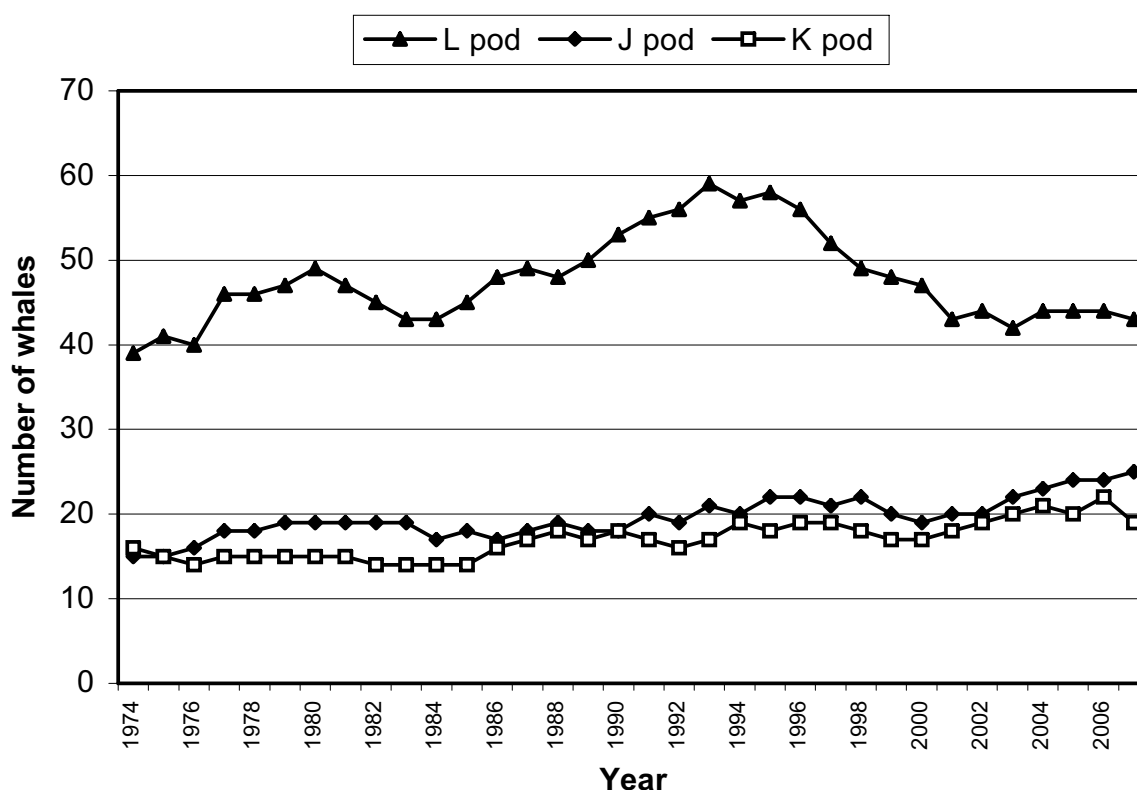
Figure 9. Population sizes and trends of the three Southern Resident killer whale pods (J, K, and L) from 1974-2007. Data were obtained through photo-identification surveys and were provided by the Center for Whale Research (unpubl. data). Data represent the number of whales present in each pod at the end of a calendar year, except for 2007, when data extend only through October (K. C. Balcomb, pers. comm.).
