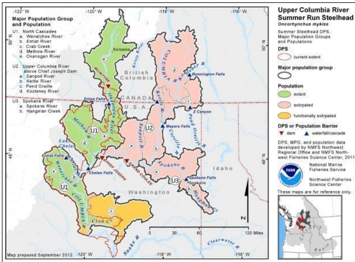
Figure 2-17. Map of the UCR Steelhead DPS's spawning and rearing areas, illustrating natural populations and MPGs (NWFS 2015).
