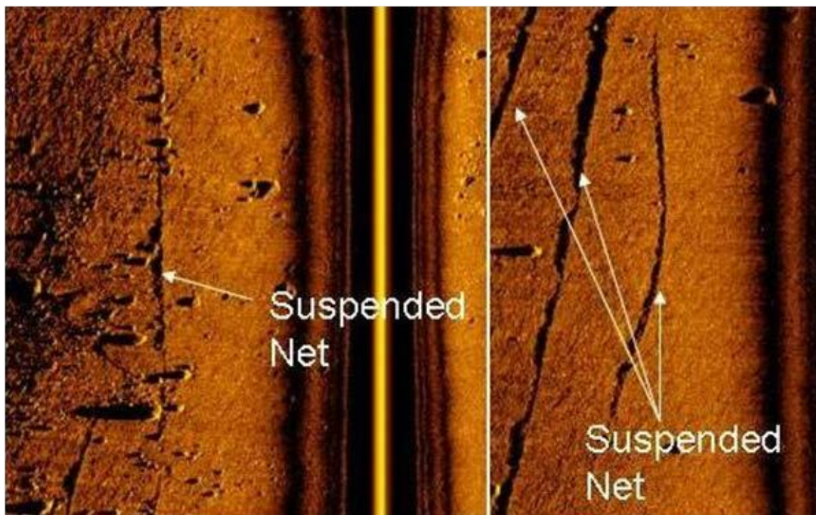
Figure 7. Sidescan sonar images of derelict nets located on Point Roberts Reef of the San Juan basin. Suspended nets have a larger acoustic shadow than nets flush with the bottom. Image used by permission of Natural Resource Consultants (NRC).
