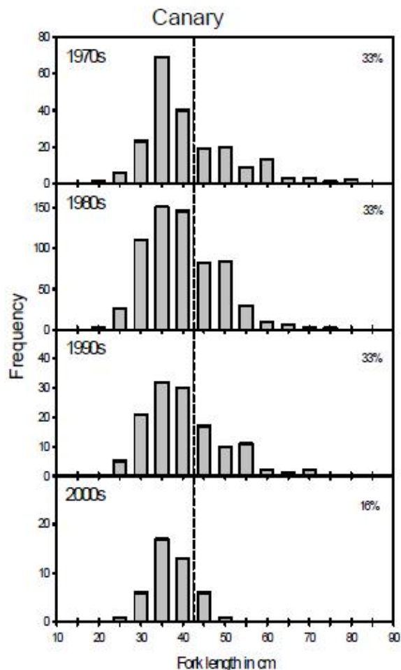
Figure 5. Canary rockfish length frequency distributions (cm) binned within four decades. The vertical line depicts the size at which about 30 percent of the population comprised fish larger than the rest of the population in the 1970s, as a reference point for later decades (figure from Drake et al. 2010b).
