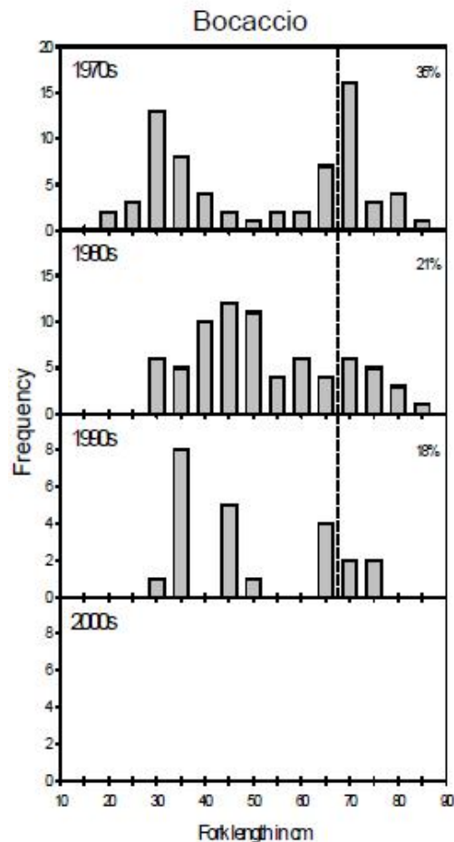
Figure 6. Bocaccio length frequency distributions (cm) binned within four decades. The vertical line depicts the size at which about 30 percent of the population comprised fish larger than the rest of the population in the 1970s, as a reference point for later decades (figure from Drake et al. 2010b).
