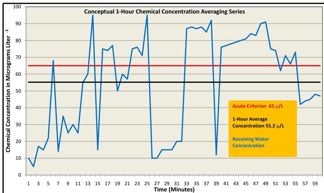
Figure A2. Conceptual concentration averaging series for acute criteria.
