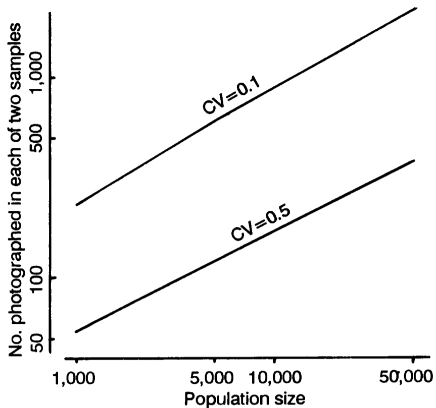
Fig. 1. The relationship between population size, the number of individuals identified in each of two samples and the coefficient of variation of a Petersen population estimate based upon the reidentification rate.
