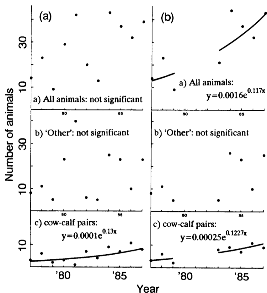
Fig. 8. Numbers seen from the aircraft, maximum in each year on one complete flight (a) Cape Leeuwin to Cape Arid (b) Cape Leeuwin to Israelite Bay. Data of Table 8; Best-fit curves of Table 9.
