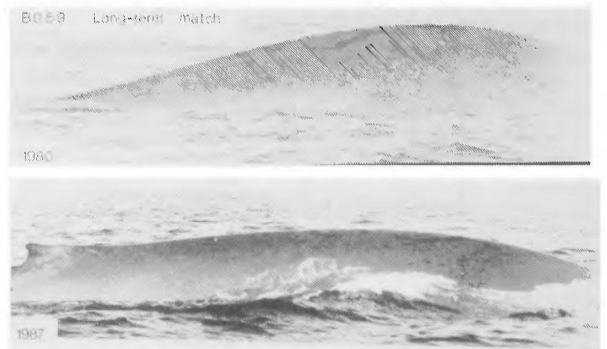
Fig. 11. Long-term match.
